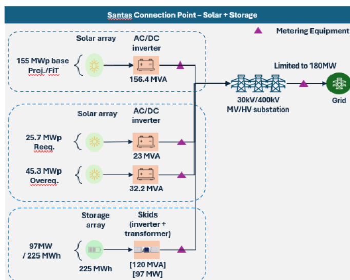
Hybridization with storage at Santas connection point
