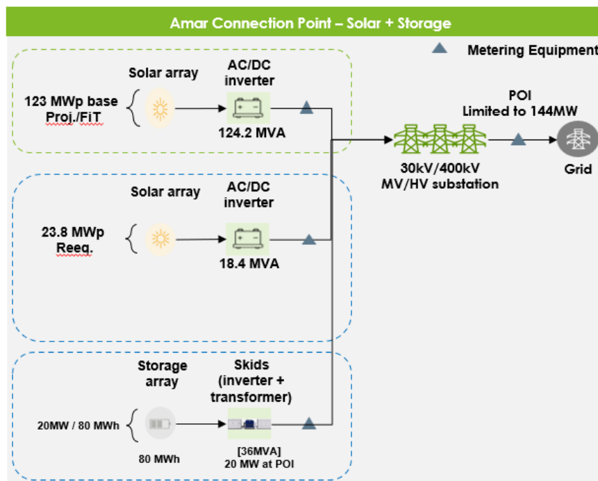
Hybridization with storage at AMAR's connection point
